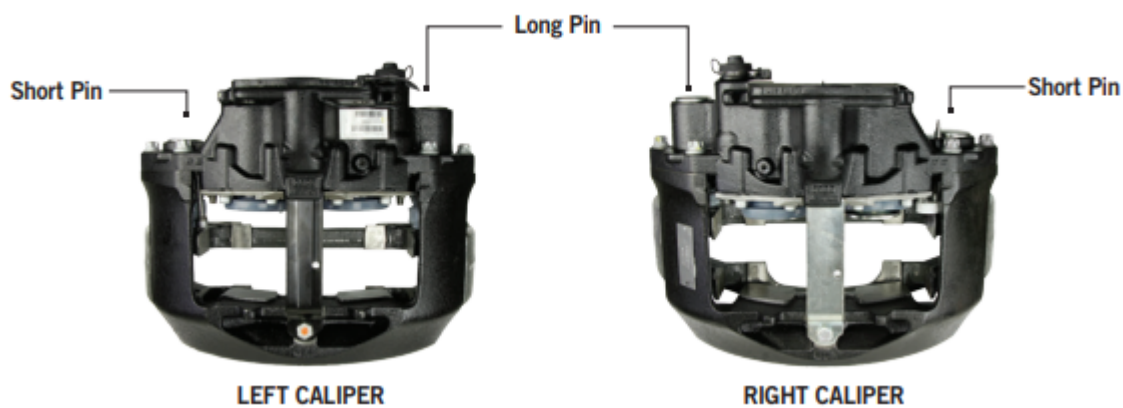
AXIAL MOUNT
