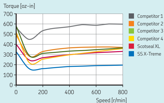
50% Friction torque reduction Torque results
